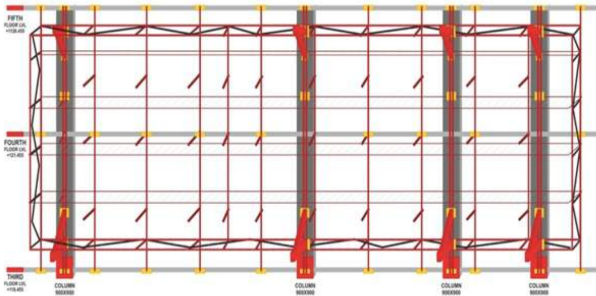
Yellow Marked MS Plate for Anchor (Mechanical/Chemical)
